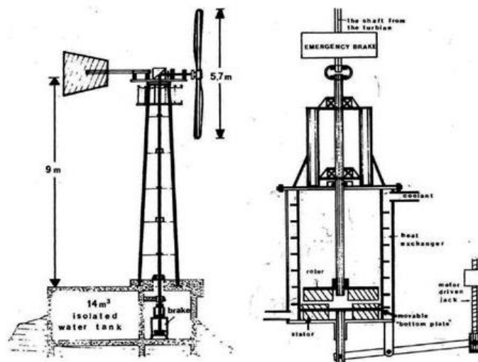
Figure 13.8 Water brake windmill developed by Ørn Helgason (left); water brake with variable load system (right) (Images: Ørn Helgason 3 ).
